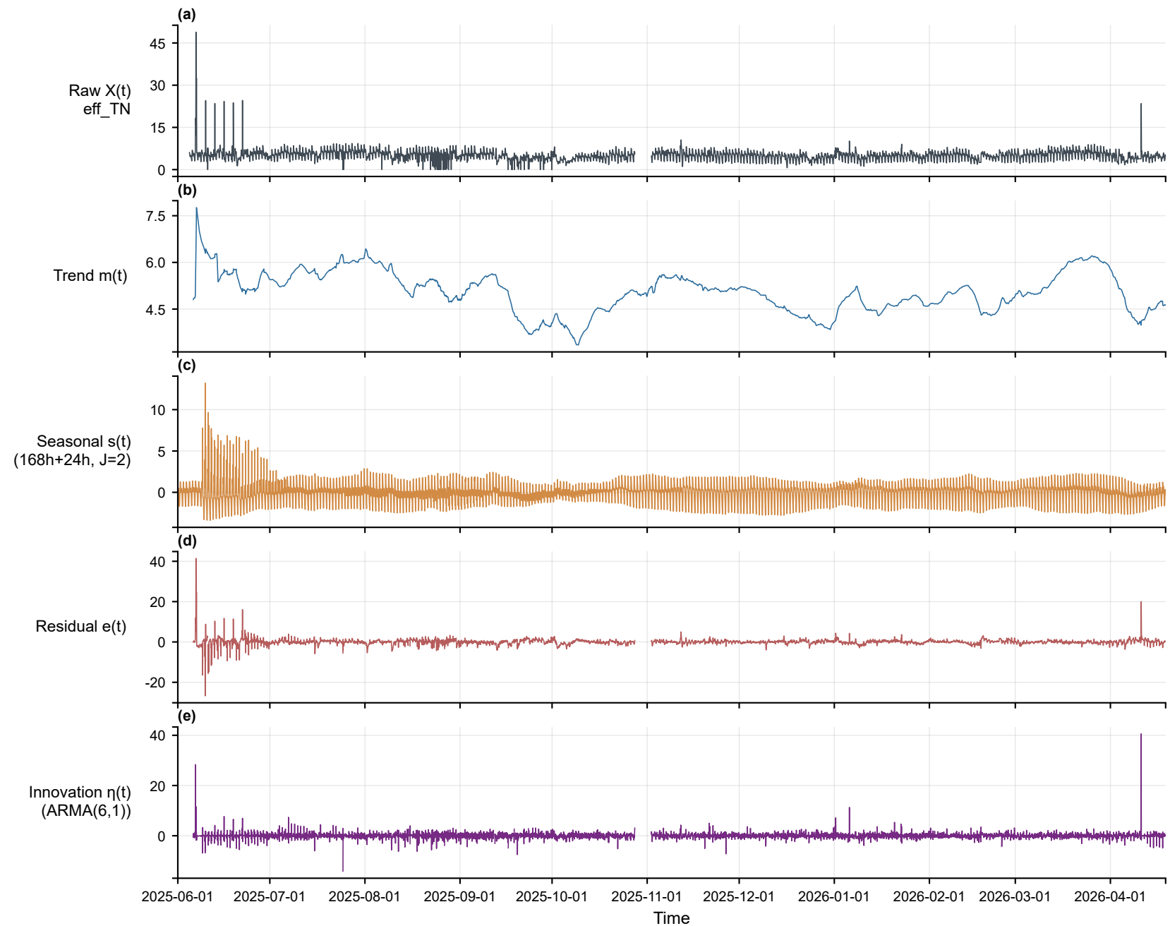
Multi-scale decomposition — eff_TN (effluent, hour) [2025-06-01~2026-04-19]
